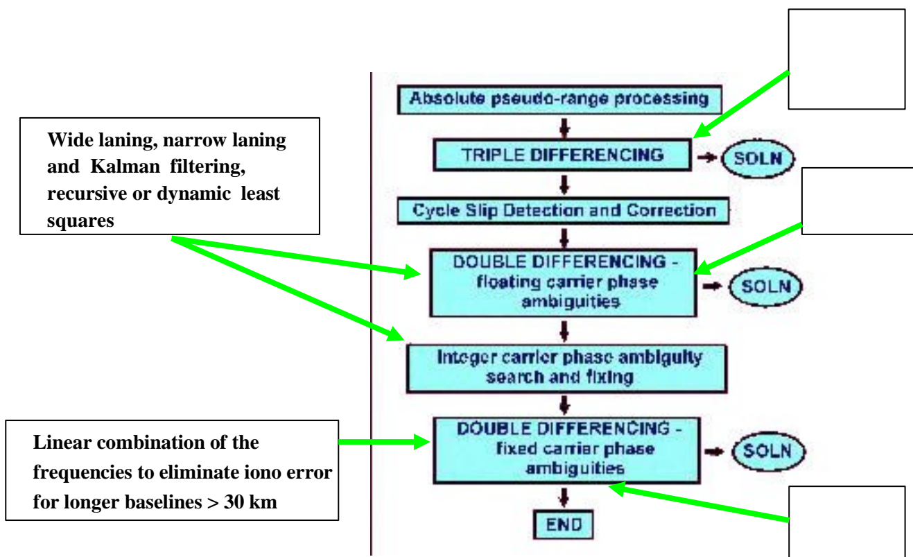
Diagram III-2 – General Flow of Ambiguity Resolution [graphic: Rizos (1999)]
